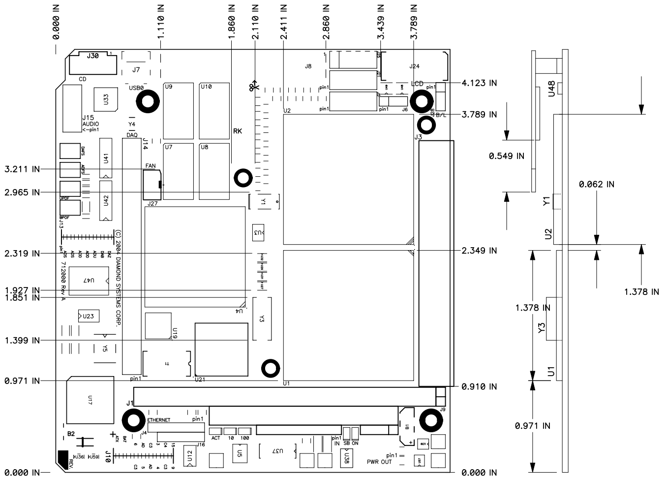
Top silkscreen
